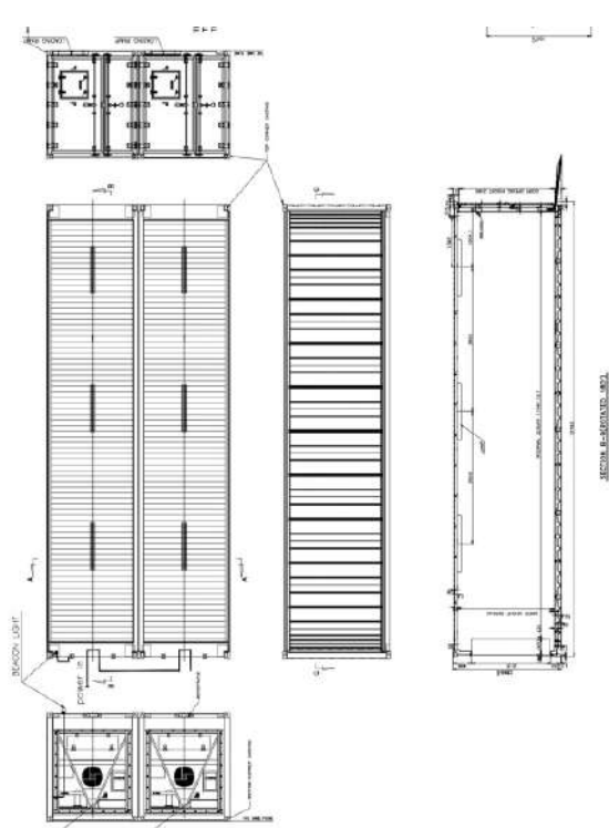
2-Bay with 2x reefers and 2x doors
