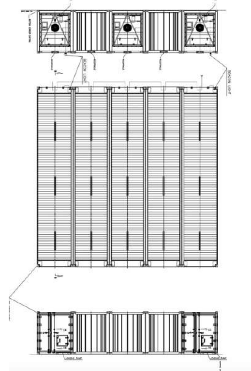
5-Bay with 3x reefers and 2x doors
